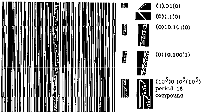
Figure 9. A simulation of example 3 with random initial conditions. The first few 'elementary' periodic points are shown at right.
