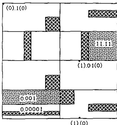
Figure 5. The period-2 and period- \delta cylinders of example 2, and its three fixed points.
