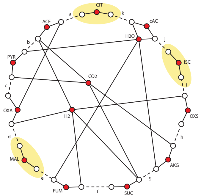
Figure B7. The projection of the TCA cycle onto CHO compounds. Phosphates and thioesters are omitted, and the stoichiometry of all acids refers to the protonated forms, so that \text{H}_2 stands for general two-electron reductants. Omission of explicit representations of substrate-level phosphorylation to form citryl-CoA and succinyl-CoA causes water elimination to accompany carboxylation of acetate and succinate in this graph, where in the actual cycle it would occur outside the graph, in the formation of pyrophosphates. Highlighted species are sole outputs and sole inputs of their associated reactions, and can be removed with the elementary composition rule (B.11) of section appendix B.2.1. Legend: acetate (ACE), pyruvate (PYR), oxaloacetate (OXA), malate (MAL), fumarate (FUM), succinate (SUC), \alpha -ketoglutarate (AKG), oxalosuccinate (OXS), cis-aconitate (cAC), isocitrate (ISC), citrate (CIT).
