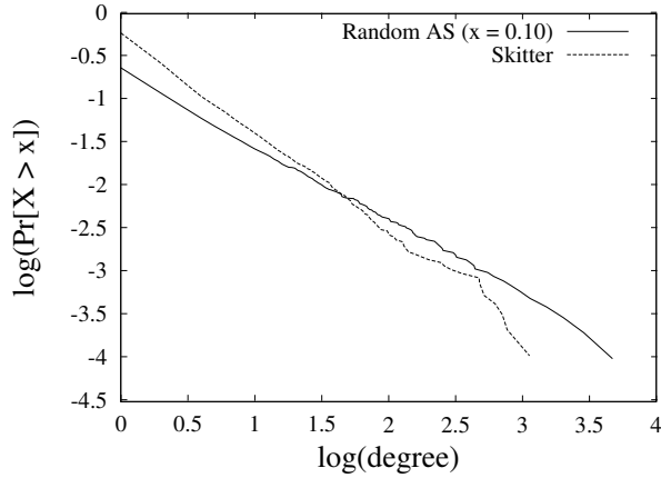
Figure 4: Predicted Degree Distribution under the Constant Connectivity Model.
