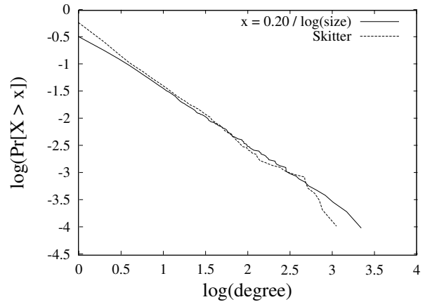
Figure 5: Validation of the Size-Based Connectivity Model.
