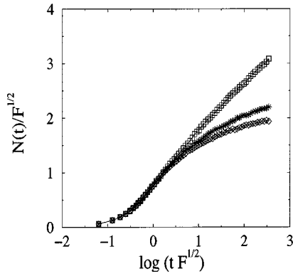
FIG. 2. Plot of N(t)/\sqrt{F} vs \log(t\sqrt{F}) for \mu=1.2 ( \diamond ), \mu=1.4 ( \star ), and \mu=2.0 ( \square ), based on simulations of point islands. The simulation parameters are the same as in Fig. 1.
