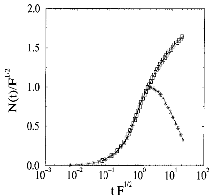
FIG. 3. Plot of N(t)/\sqrt{F} vs t\sqrt{F} for \mu=1.2 and F=0.001 for point ( \square ) and growing circular islands ( \star ).
