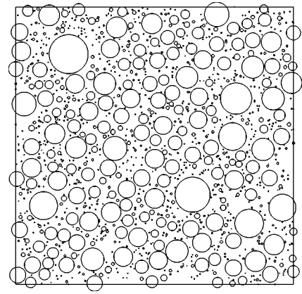
FIG. 4. Central portion of a typical droplet configuration for \mu=1.2 and F=0.001 for a system of size 500 \times 500 .
