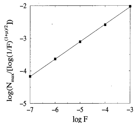
FIG. 5. Plot of \log[N_{\text{max}}/[\log(1/F)]^{(1+\mu/2)}] vs \log(F) for \mu=1.2 . The slope of the line is 0.53.
