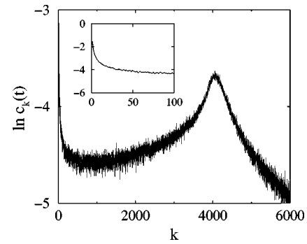
FIG. 1. Semilogarithmic plot of \ln c_k(t) vs k at t \approx 22000 for \mu = 1.5 based on simulations of point islands. The data are based on 5000 realizations of an initially empty system of 2000 sites with F = 0.05 . Notice the existence of an inner scale k \approx \kappa \approx 50 (inset), and an outer scale for k \approx K \approx 4000 .
