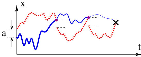
Figure 1. Space-time evolution of a single mosquito (dashed) and man (solid). After each encounter, the mosquito is displaced by \pm a with respect to the man, while the man becomes progressively more sluggish and eventually comes to rest.
