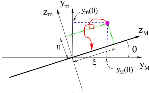
Figure 2. Mapping the diffusion of a man and mosquito on the line to diffusion in the half space z_m > 0 . A first-passage trajectory is shown.
