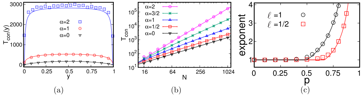
Figure 5. (a) Consensus time versus y . Equation (22) gives the curves and symbols represent simulation results for N = 128 voters over 10^4 realizations. (b) Consensus time versus N . The curves again represent the predictions from equation (22). We fix \ell = 1 and use \alpha = p/(1 - p) to specify p for a given \alpha value. (c) Consensus time exponent versus p for two \ell values. The symbols represent simulation results and the curves are predictions from equation (23).
