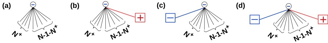
Figure A1. Possibilities for a - voter (circle) to be connected to the news sources (squares). (a) The - voter is connected to N - 1 neighboring voters, with N^+ having + opinion, but not to any news source. (b) The - voter is connected to a + news source, (c) connected to the - news source, and (d) connected to both the news sources.
