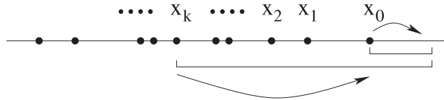
Figure 1. Stochastic rat race model. Each particle has a fitness x_k . The leader can advance by an amount that is uniformly distributed in the range x_0 - x_1 . The k th particle can advance by an amount that is uniformly distributed in m(x_0 - x_k) .
