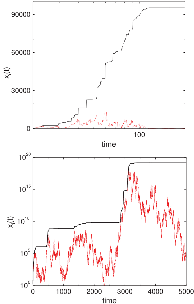
Figure 5. Fitnesses of each agent for a six-particle system for m = 1.61 on a log-linear scale (top) and m = 1.64 on a linear-log scale (bottom). Shown dotted is the distance between the strongest and weakest agent.
