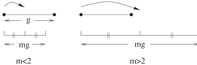
Figure 3. Deterministic rat race. The laggard advances by mg/2 . For m < 2 , the order never changes, while for m > 2 , the move of the laggard always leads to passing.
