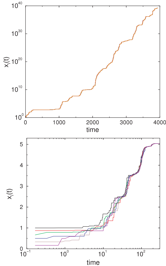
Figure 4. Fitnesses of each agent for a six-particle system for m = 0.4 on a linear-log scale (top), and m = 0.44 on a log-linear scale (bottom).
