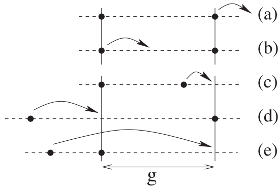
Figure 2. Advancement events that contribute to the change in the gap length for a two-particle rat race. Gaps of length g are lost by the first two process, while the latter three lead to a gain of gaps of length g . The last process is a lead-changing event.
