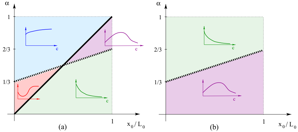
Figure 2. Splitting probability phase diagram for the (a) contracting and (b) expanding cage in the speed ratio ( \alpha ) and initial position ( x_0 ) plane. In (a), \mathcal{L}^c \approx 1 for c \rightarrow \infty above the solid line, while \mathcal{L}^c \approx 0 for c \rightarrow \infty below. Above the dashed line \mathcal{L}^c is an increasing function of c at c = 0 and a decreasing function below. These lines delineate four zones of behavior as discussed in the text. In (b), there are two zones.
