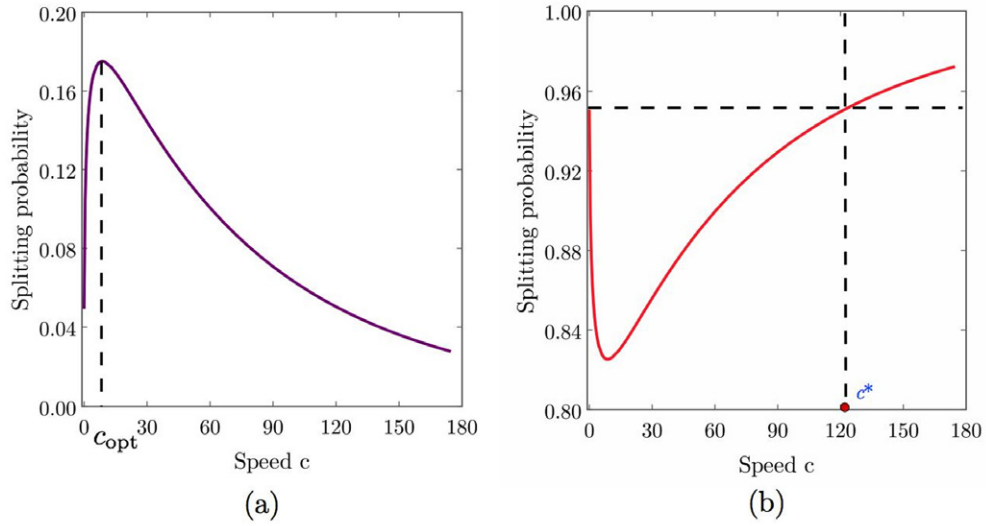
Figure 3. Splitting probability to catch the lamb in the (a) ‘optimizable zone’ and (b) ‘dilemma zone’. In (a), the splitting probability is increased substantially (by more than a factor 3 for \alpha = 0.92 , x_0 = 19 , and L_0 = 20 ) when the shepherd moves at the optimal speed c_{\text{opt}} instead of staying still. In (b), the probability to catch the lamb is diminished if the shepherd runs slower than speed c^* . Here the parameter values are \alpha = 0.08 , x_0 = 1 and L_0 = 20 .
